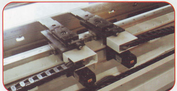
Servo Controlled Back Gauge Fingers(Z1, Z2)
