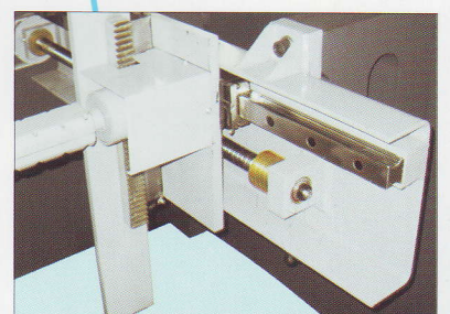
"Rexroth" ball screw and linear guide way
